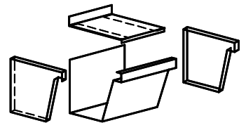
Expansion Joint
