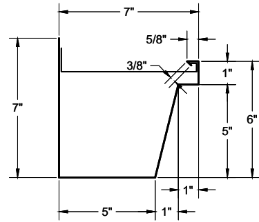
Custom Smacna "F" Gutter (___ Stretchout)
